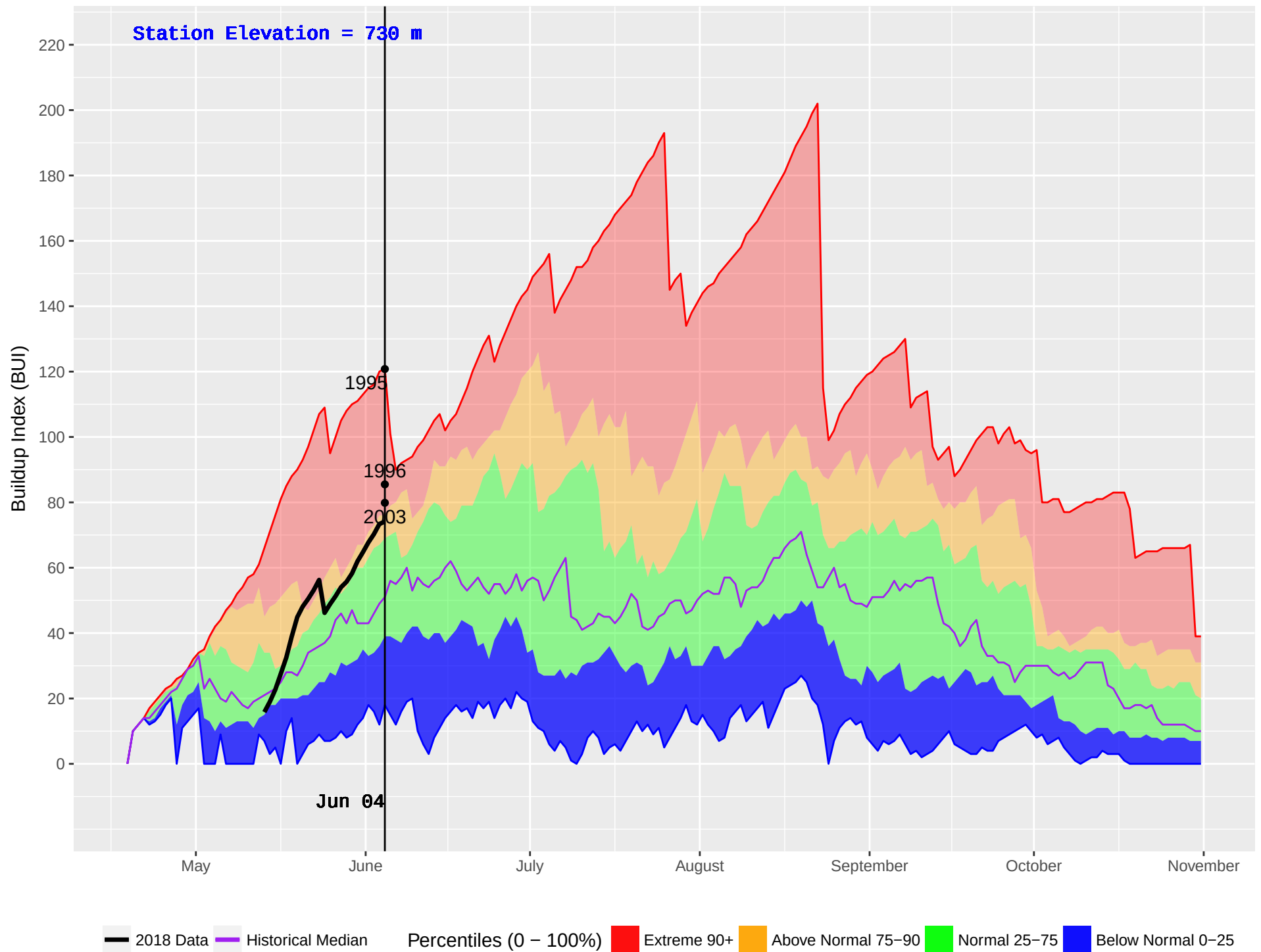
BOYA LAKE (445) : Historical (1985–2016) and Current (2018) Noon Buildup Index (BUI)
