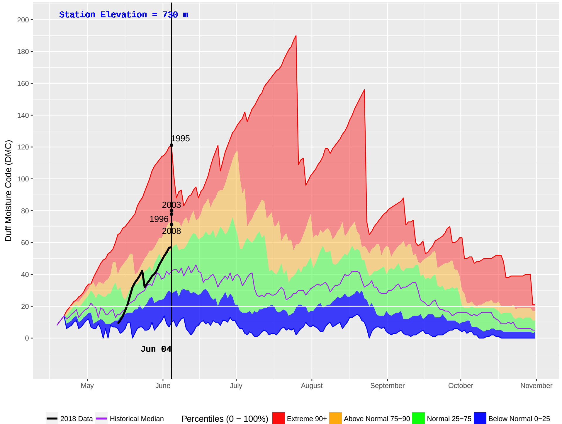
BOYA LAKE (445) : Historical (1985–2016) and Current (2018) Noon Duff Moisture Code (DMC)
