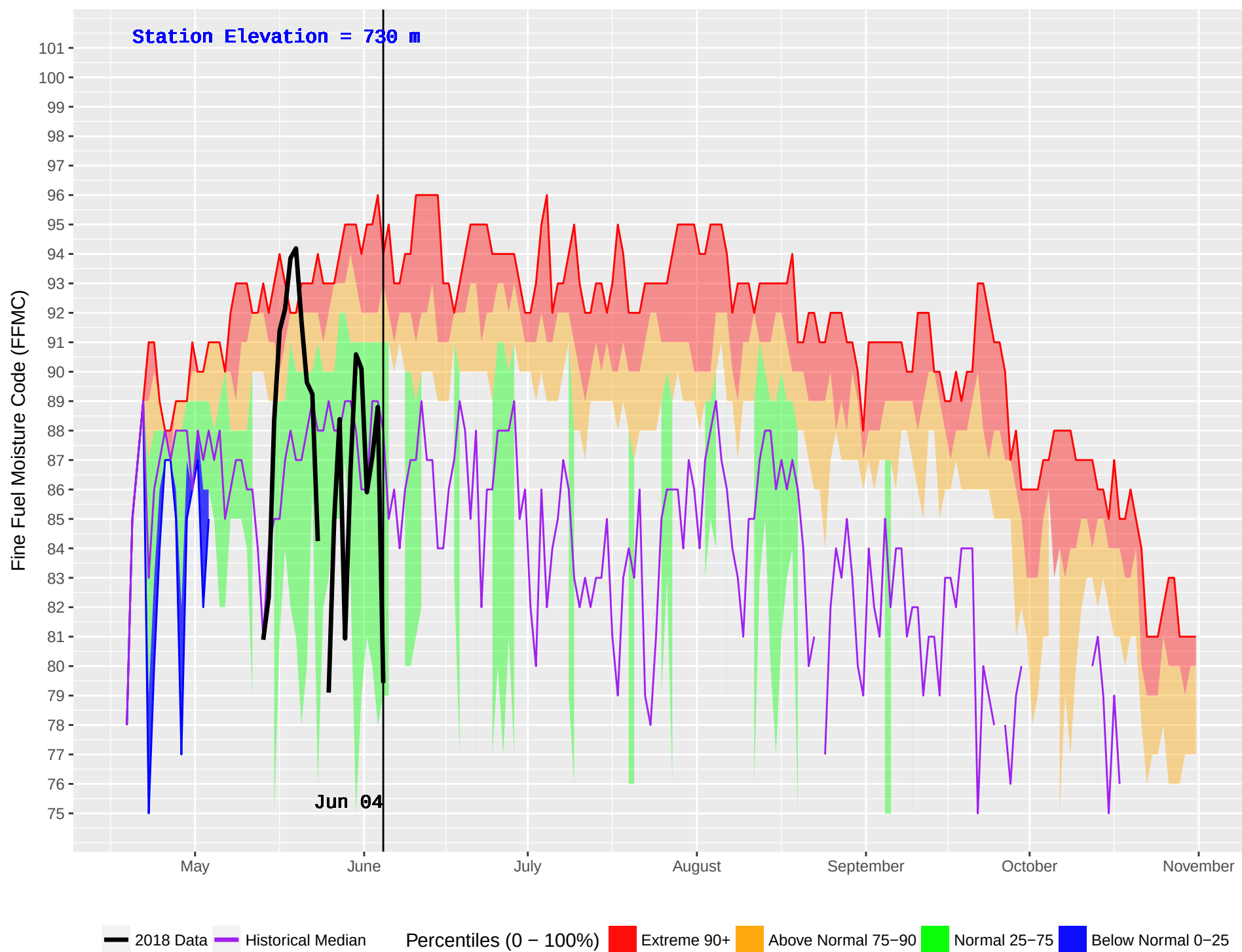
BOYA LAKE (445) : Historical (1985–2016) and Current (2018) Noon Fine Fuel Moisture Code (FFMC)
