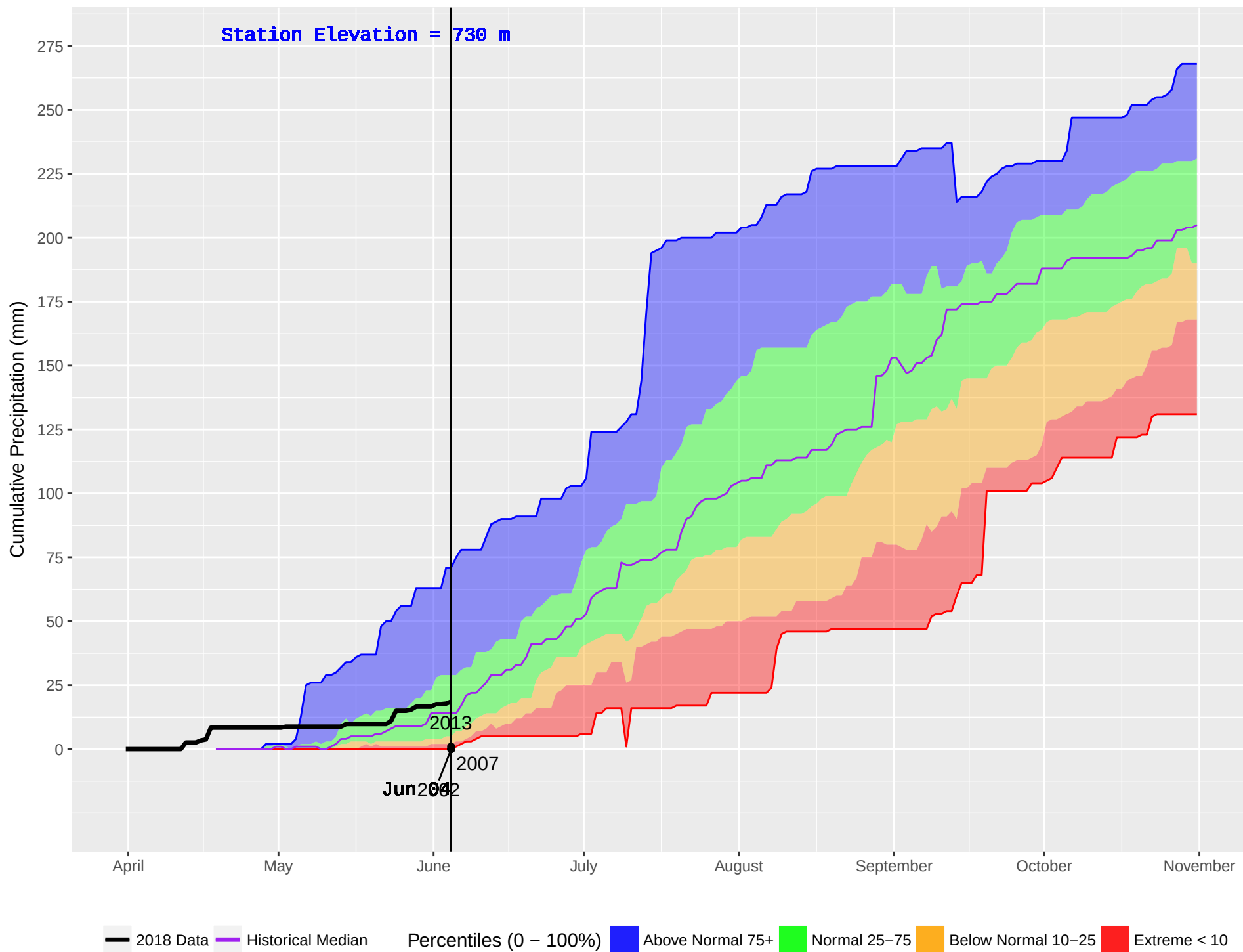
BOYA LAKE (445) : Historical (1985–2016) and Current (2018) Noon Cumulative Precipitation
