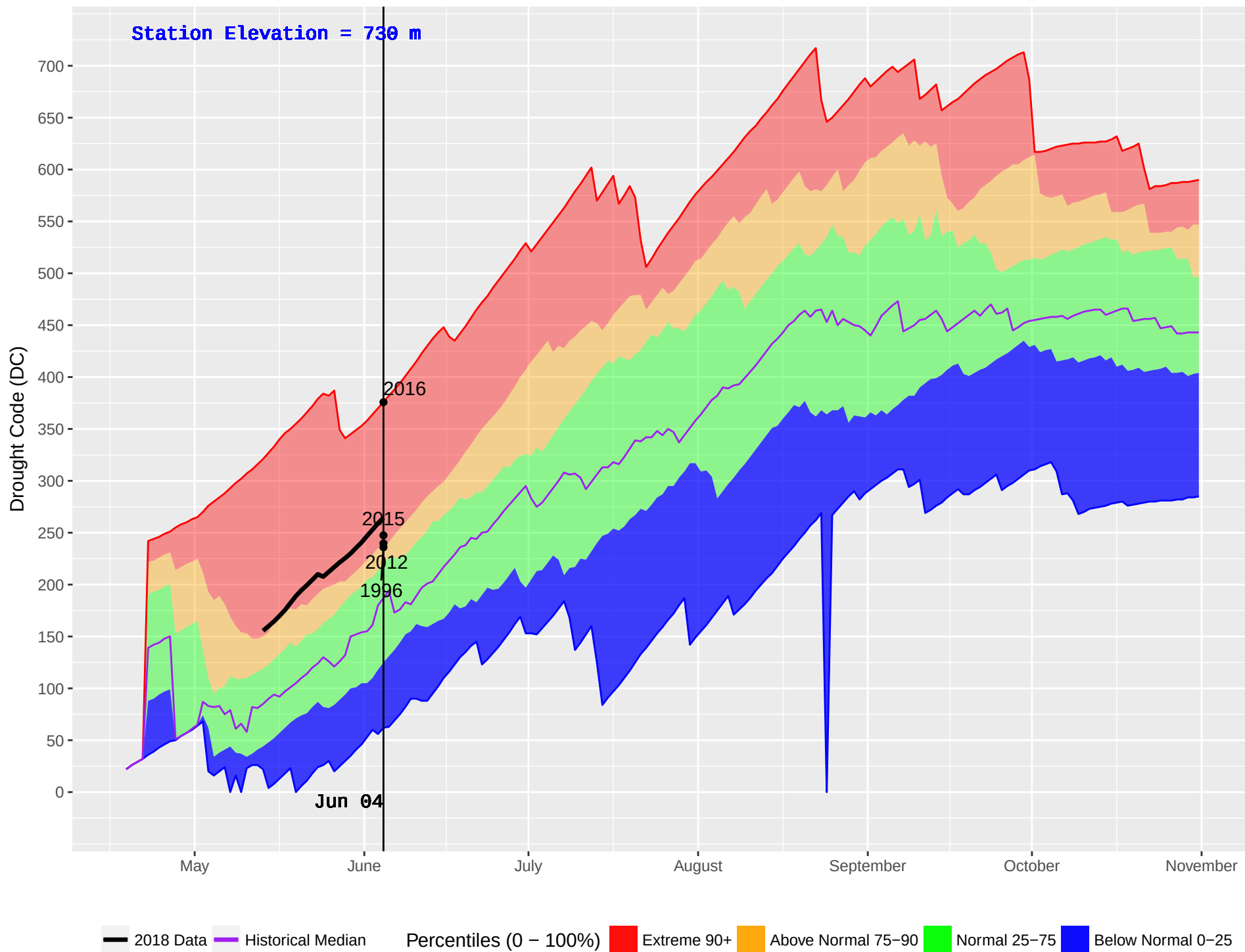
BOYA LAKE (445) : Historical (1985–2016) and Current (2018) Noon Drought Code (DC)
