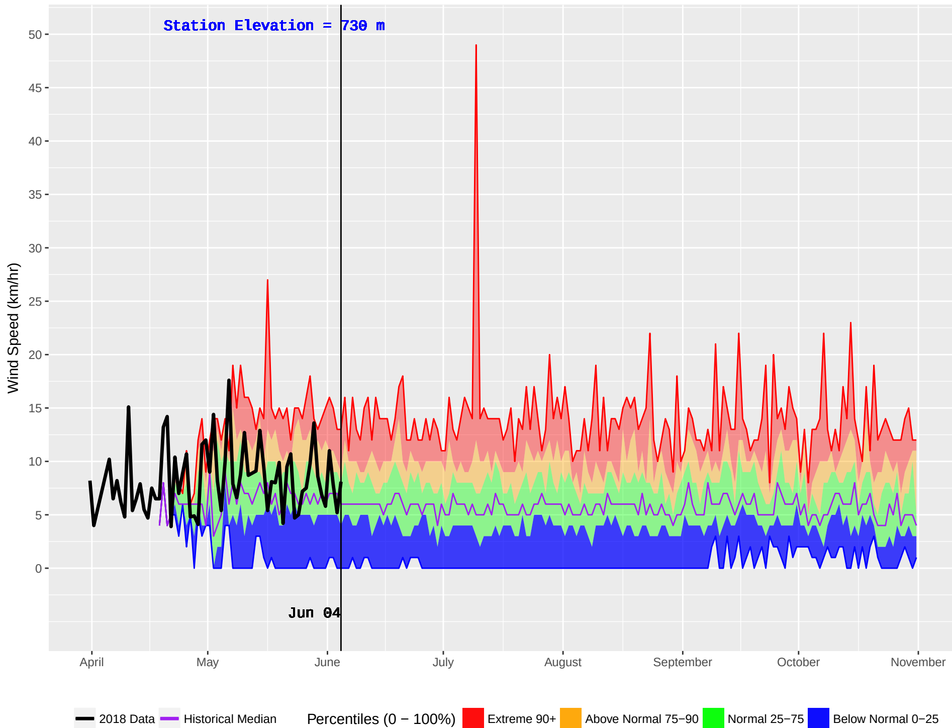
BOYA LAKE (445) : Historical (1985–2016) and Current (2018) Noon Wind Speed
