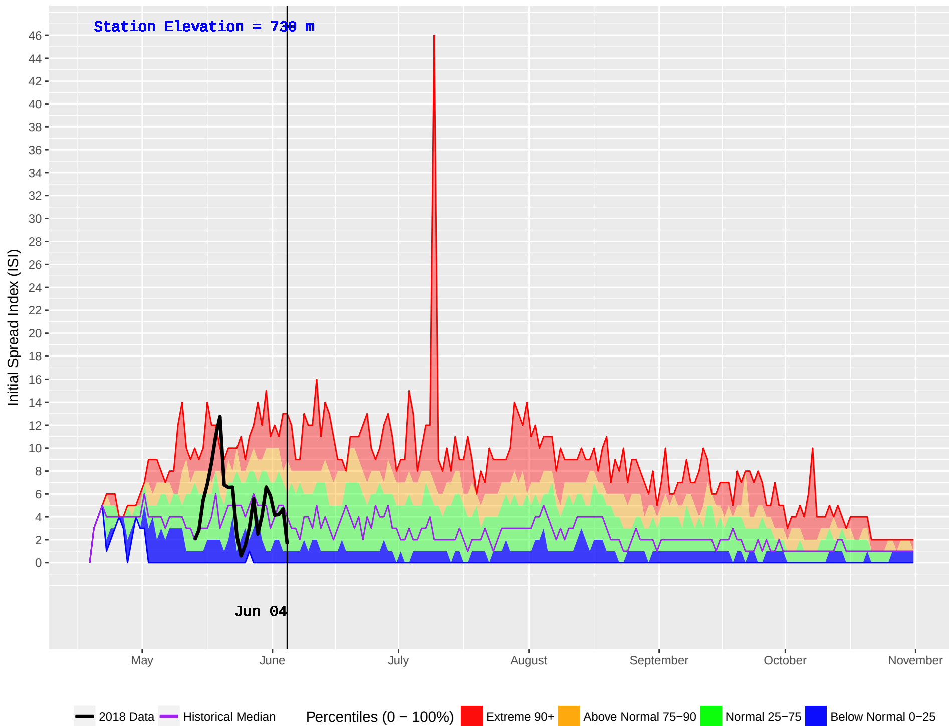
BOYA LAKE (445) : Historical (1985–2016) and Current (2018) Noon Initial Spread Index (ISI)
