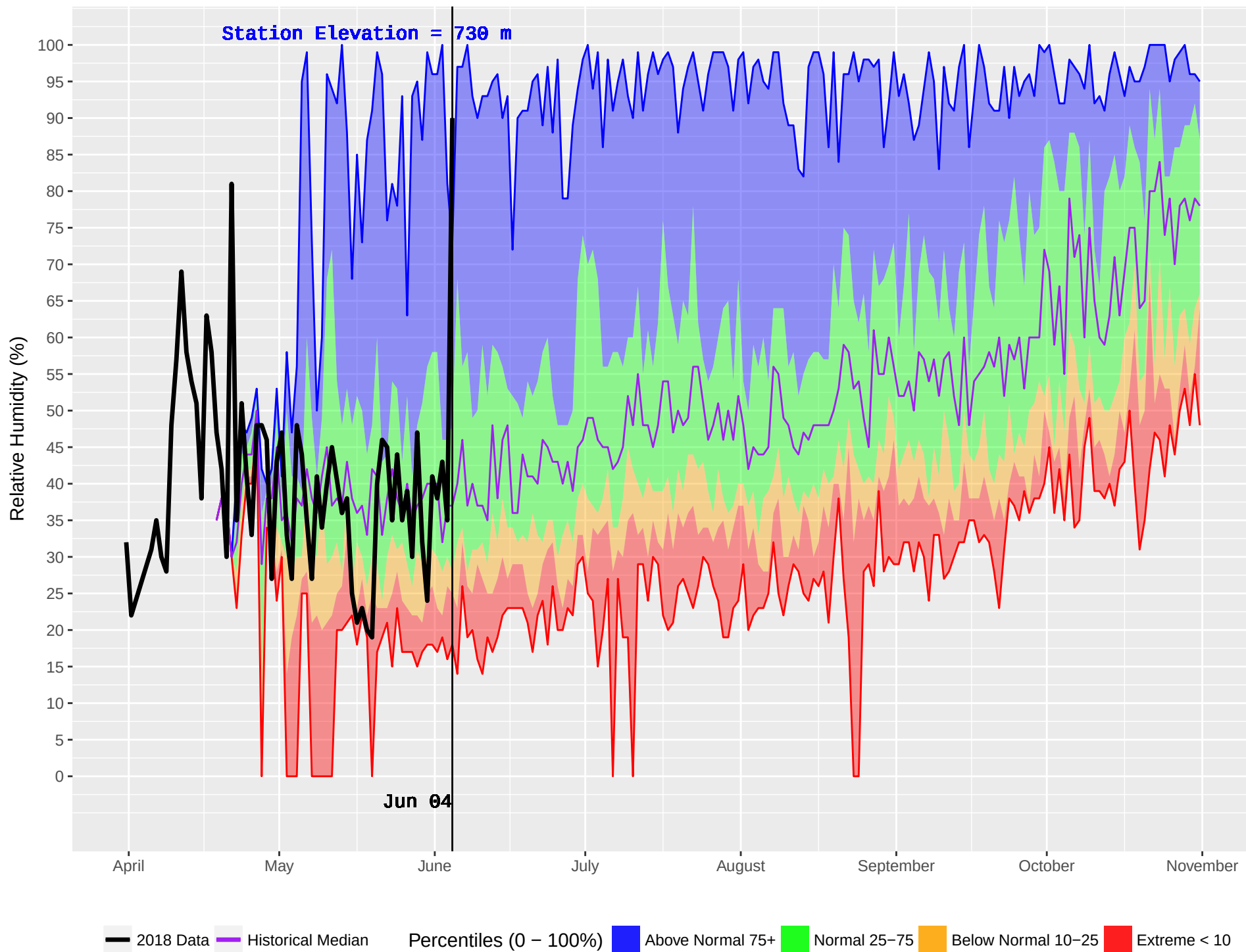
BOYA LAKE (445) : Historical (1985–2016) and Current (2018) Noon Relative Humidity
