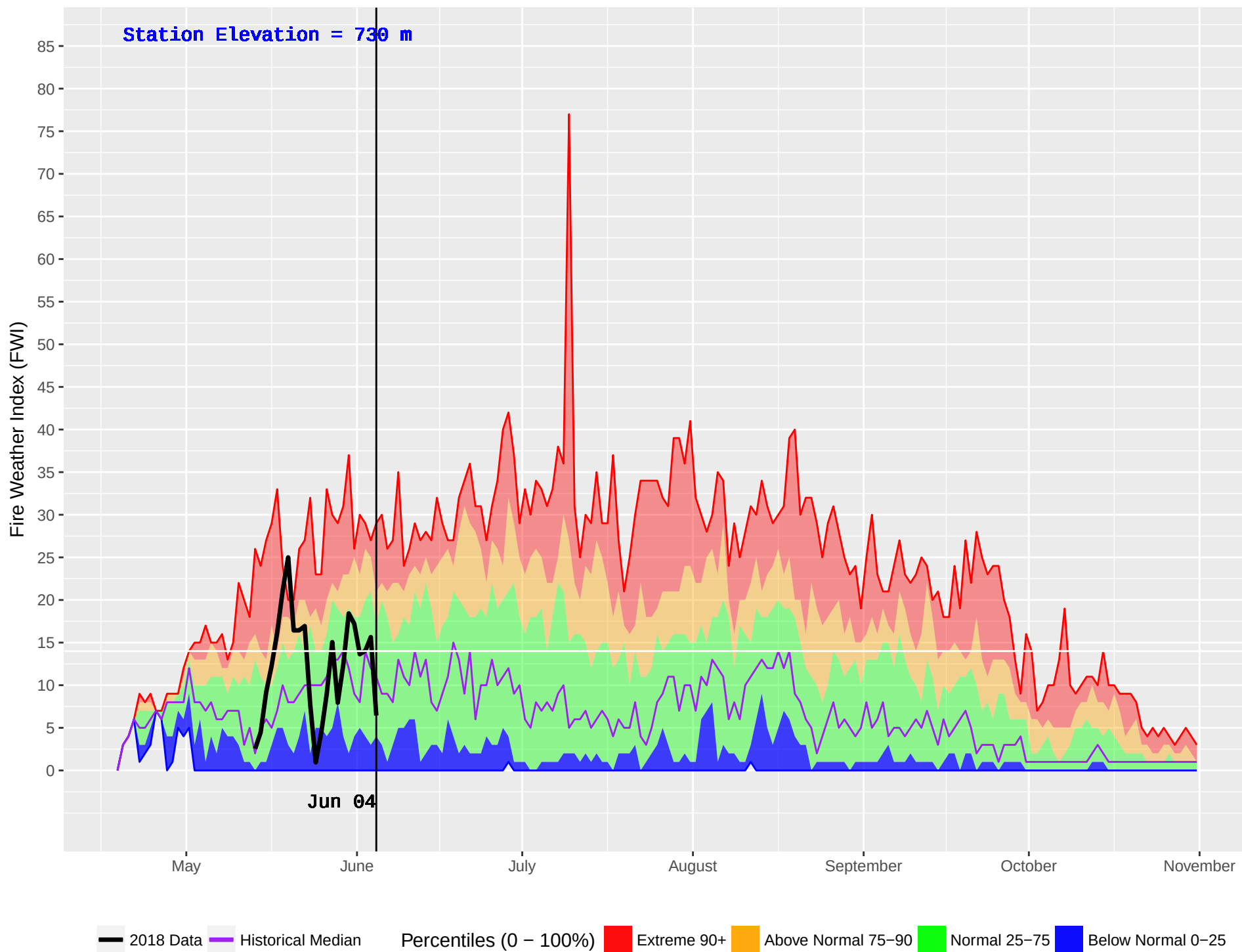
BOYA LAKE (445) : Historical (1985–2016) and Current (2018) Noon Fire Weather Index (FWI)
