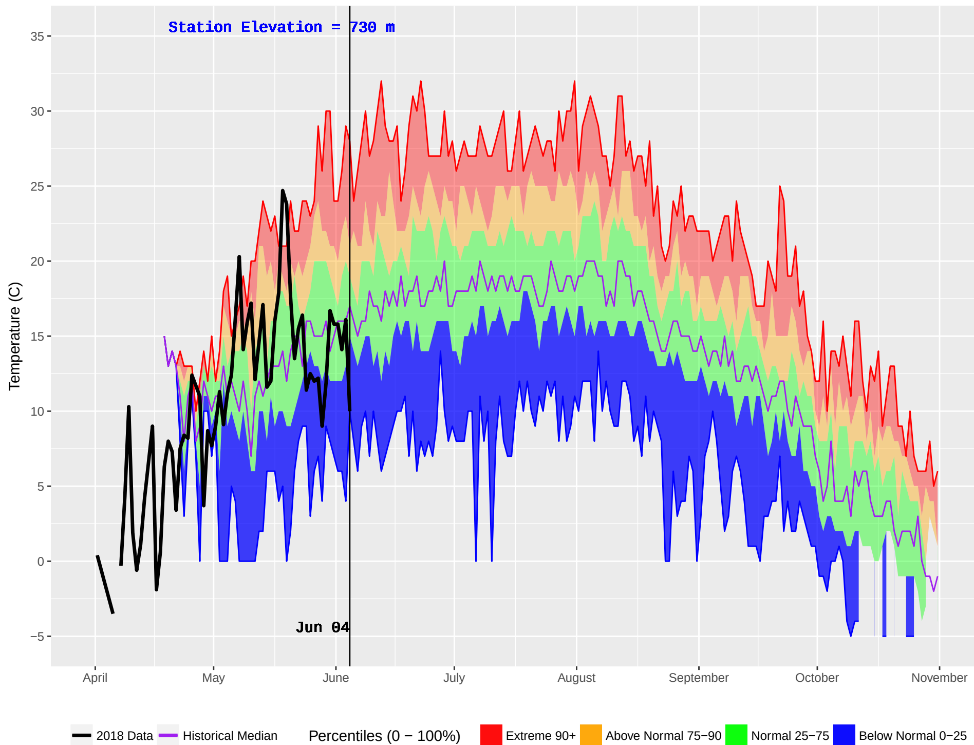
BOYA LAKE (445) : Historical (1985–2016) and Current (2018) Noon Temperature
